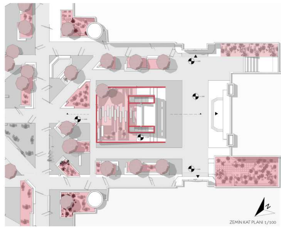
ZEMİN KAT PLANI 1/100
